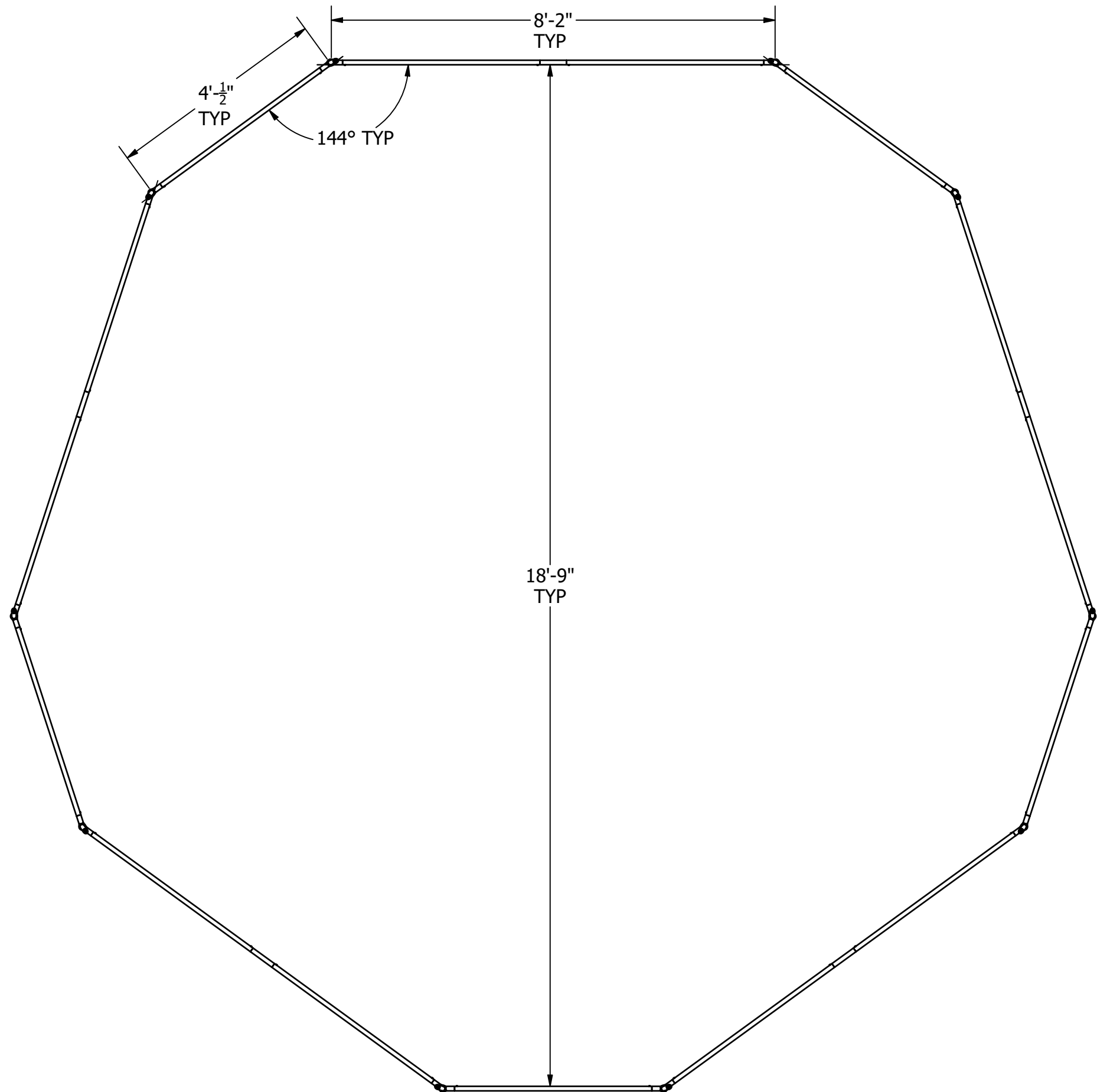
DOME FOOTPRINT-INTERIOR DIMENSIONS AREA- 284 SQ FT
